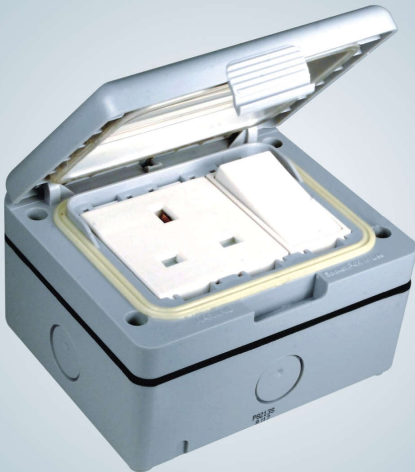
P8213S IP55 13A 1 Gang switched Socket
